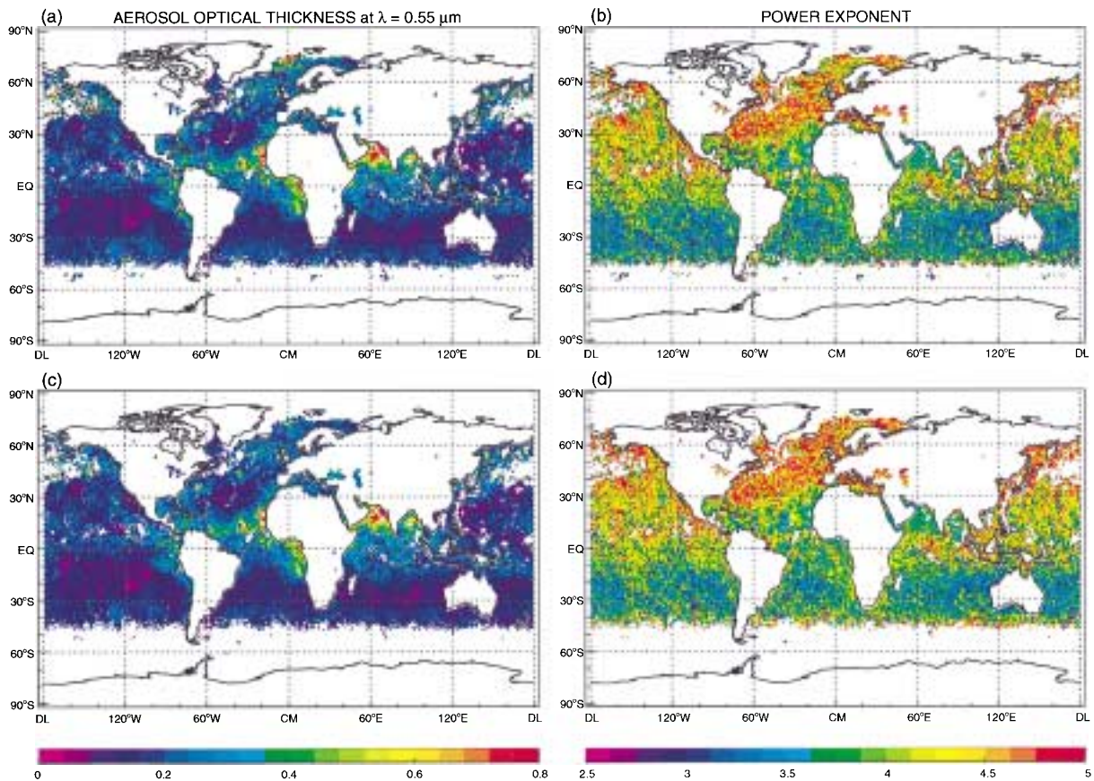
Fig. 7. (a) and (b) As in panels (a) and (b) of Fig. 6 but with the cloud-detection scheme that retains only pixels with channel-5 temperatures warmer than their composite counterparts by 1 K or more. (c) and (d) As in panels (a) and (b) but with the addition of the S_{12} threshold.
