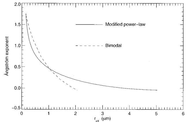
Fig. 4. Ångström exponent versus effective radius for the power-law size distribution of Eq. (4) and the bimodal size distribution of Eq. (11).
