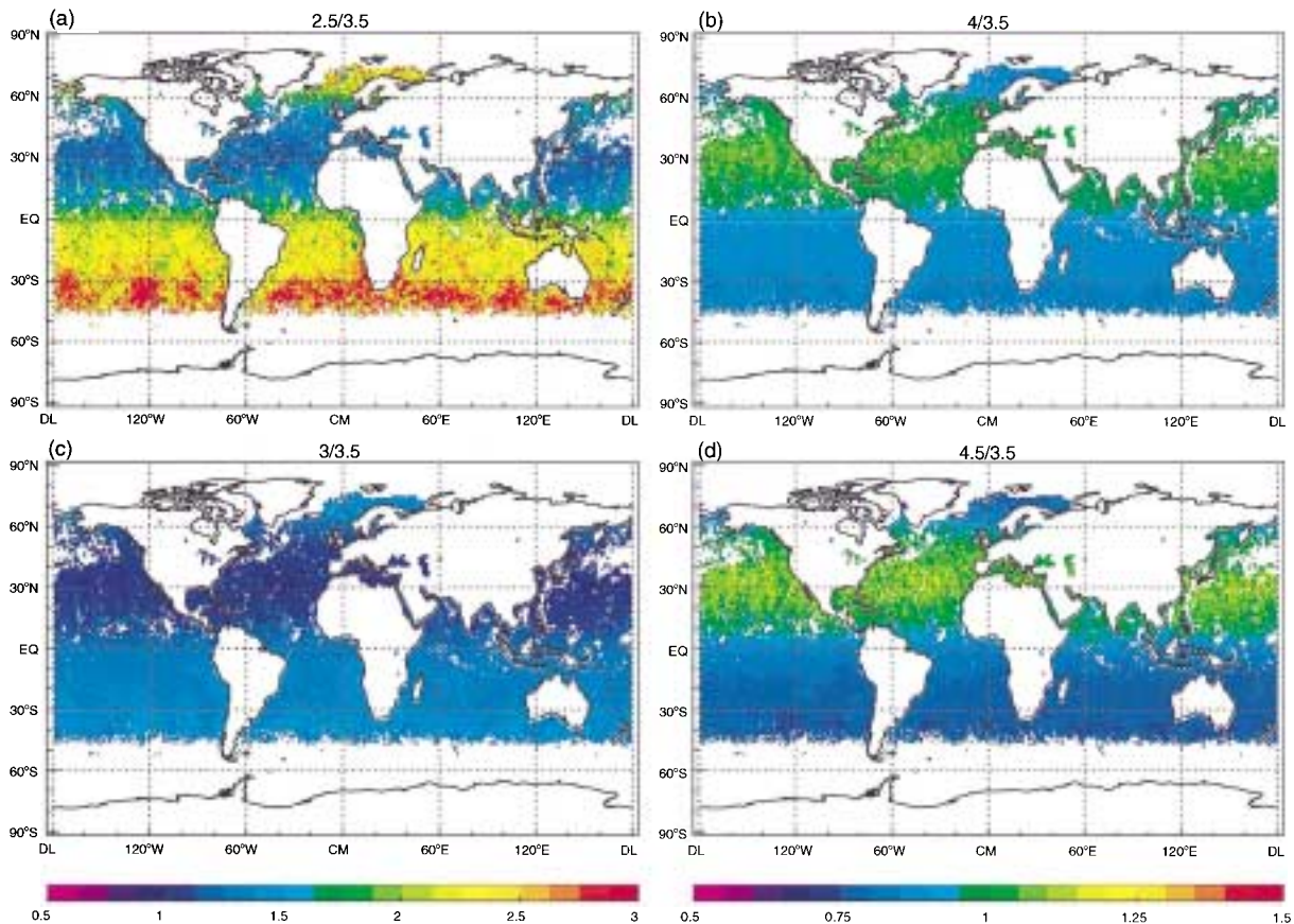
Fig. 18. Aerosol optical thickness retrieved with the one-channel algorithm based on the power-law size distribution of Eq. (4) with \alpha = 2.5, 3, 4, and 4.5 relative to that retrieved for \alpha = 3.5 for July 1986.
