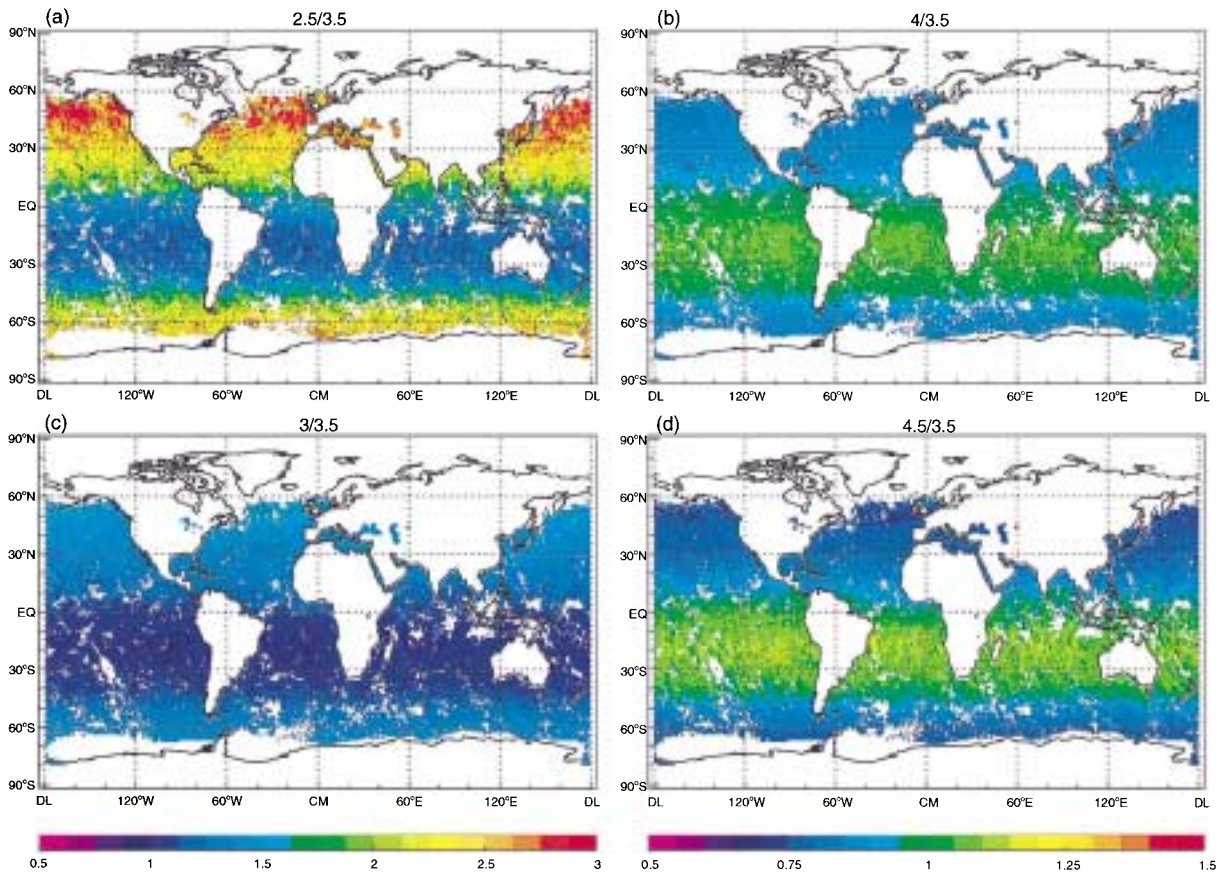
Fig. 19. As in Fig. 18 but for January 1986.
