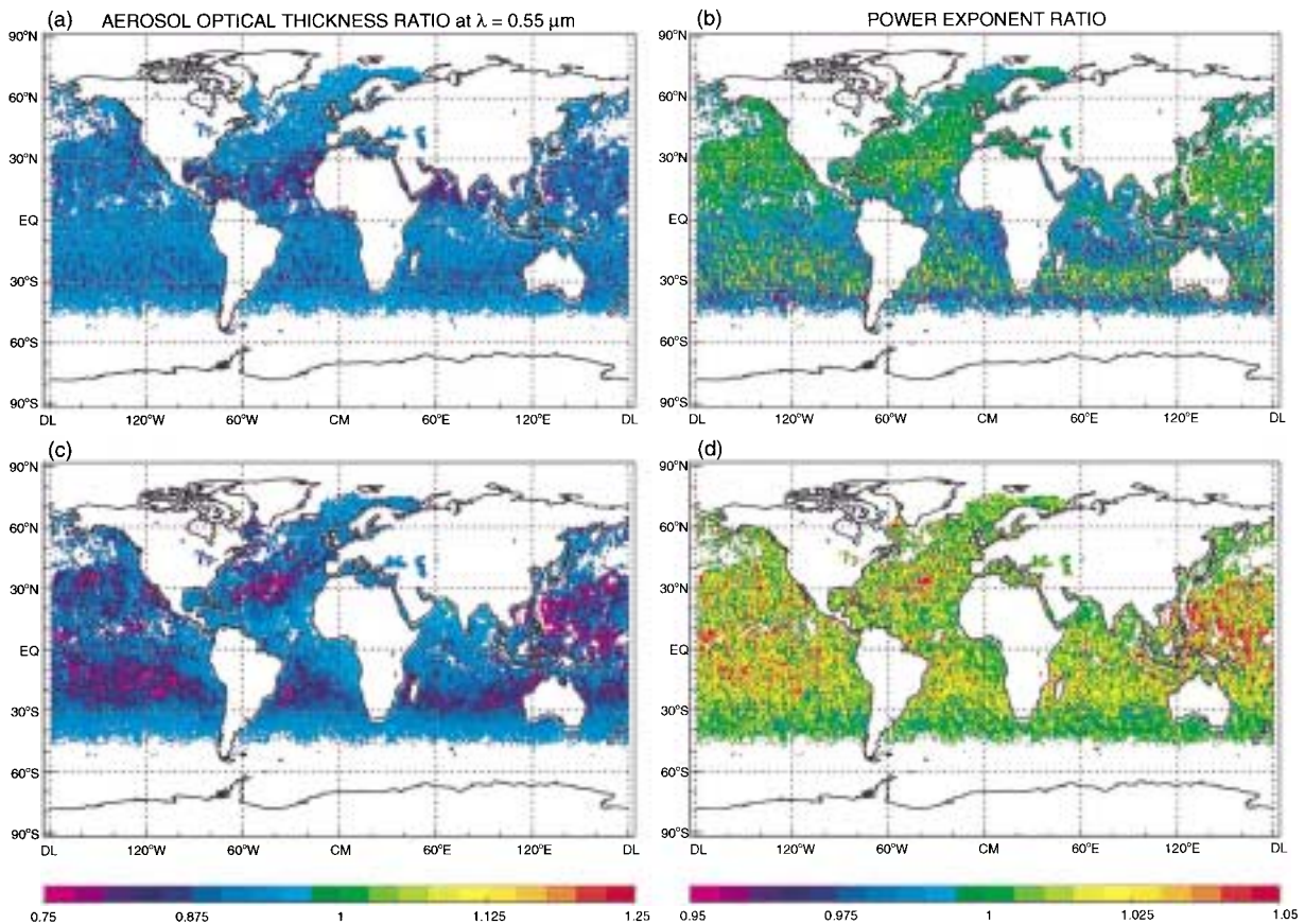
Fig. 11. (a) and (b) Ratios of the mean optical thickness and power exponent retrieved assuming the refractive index m = 1.5 + 0.002i relative to those shown in Figs. 7(c) and 7(d), respectively. (c) and (d) Ratios of the mean optical thickness and power exponent retrieved assuming a small added diffuse contribution to the ocean reflection function relative to those shown in Figs. 7(c) and 7(d), respectively.
