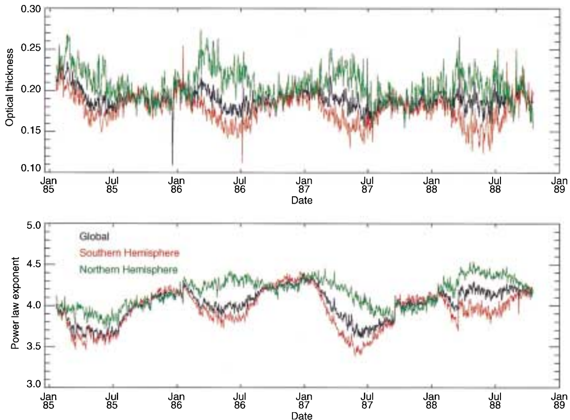
Fig. 8. Global and hemisphere averages of the aerosol optical thickness and power exponent plotted with daily resolution. Horizontal ticks correspond to the 15th day of the respective months.
