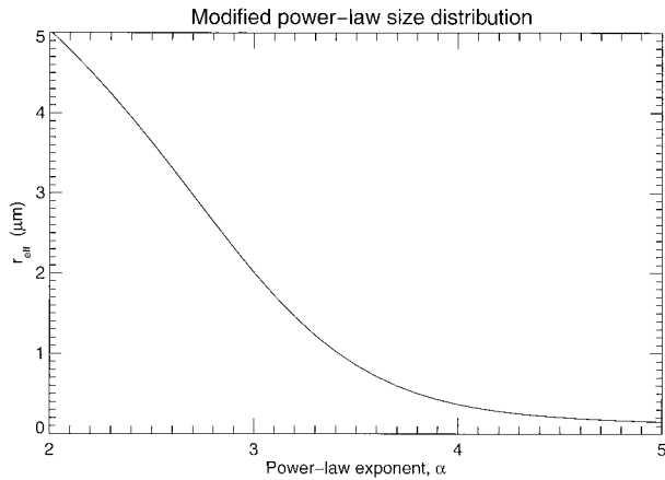
Fig. 2. Effective radius versus power exponent for the power-law size distribution of Eq. (4).
