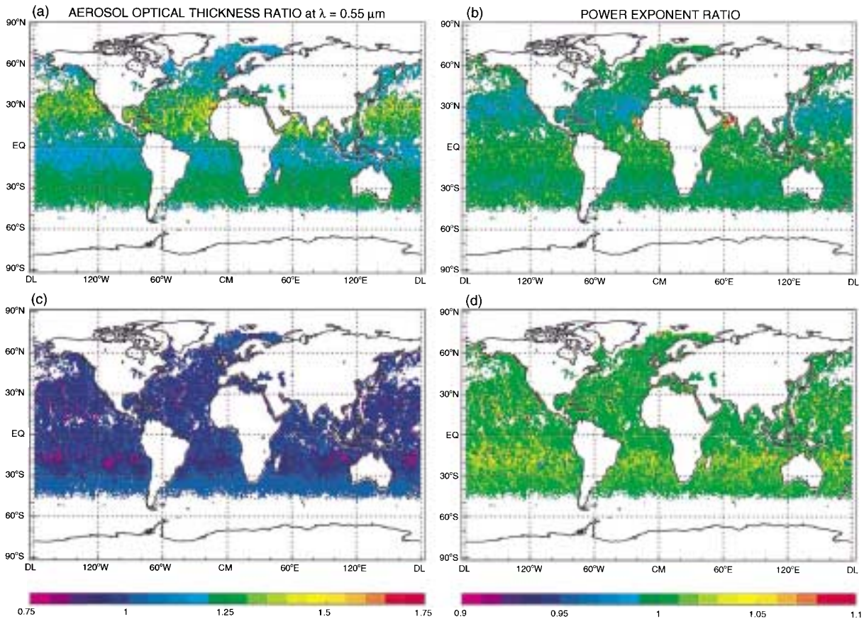
Fig. 13. (a) and (b) Ratios of the mean optical thickness and power exponent retrieved assuming the refractive index m = 1.4 + 0.005i relative to those shown in Figs. 7(c) and 7(d), respectively. (c) and (d) Ratios of the mean optical thickness and power exponent retrieved assuming a wind speed of W = 11 m/s relative to those shown in Figs. 7(c) and 7(d), respectively.
