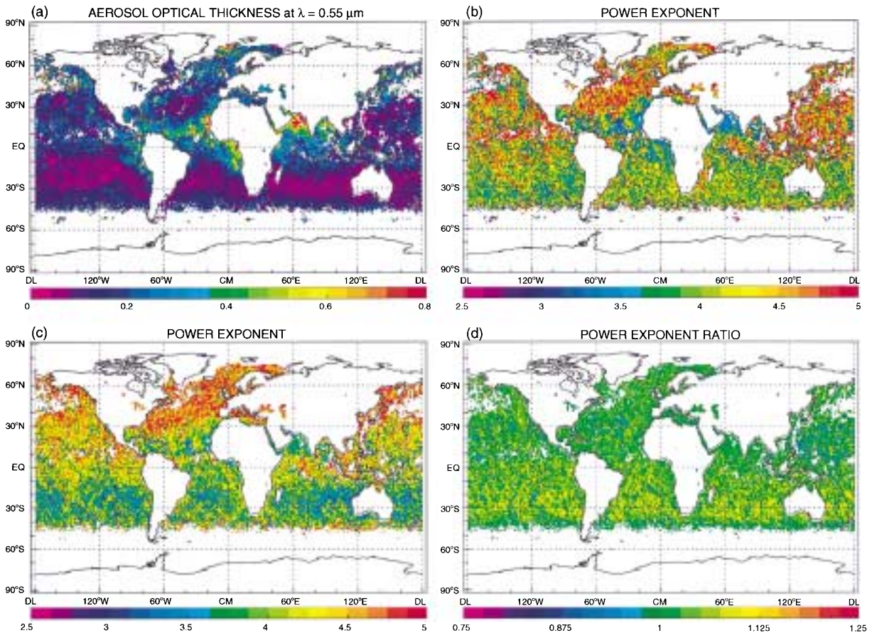
Fig. 9. (a) and (b) As in panels (a) and (b) of Fig. 7 but with the NOAA postlaunch calibration of NOAA-9 AVHRR channels 1 and 2. (c) As in panel (d) of Fig. 7 but for \bar{\alpha} . (d) \bar{\alpha}:\langle\alpha\rangle ratio.
