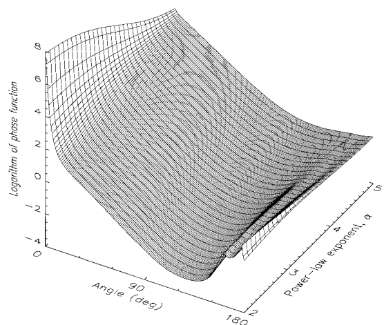
Fig. 12. Phase function versus power exponent and scattering angle for the power-law size distribution of Eq. (4) and m = 1.5 + 0.002i .
