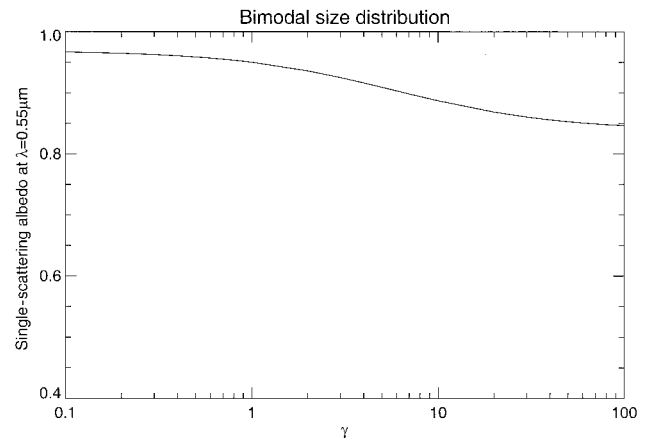
Fig. 17. Single-scattering albedo versus \gamma for the bimodal log normal size distribution of Eq. (11) and m = 1.5 + 0.005i .
