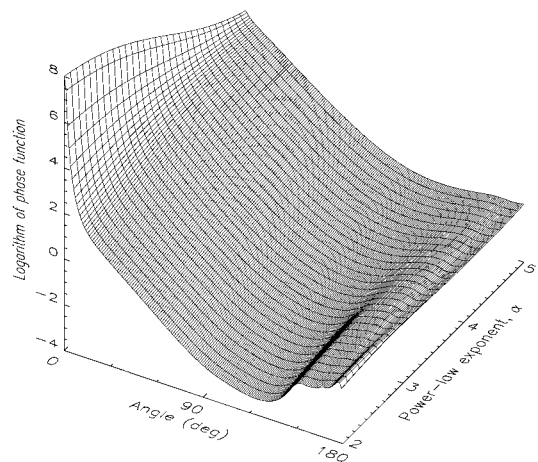
Fig. 14. Phase function versus power exponent and scattering angle for the power-law size distribution of Eq. (4) and m = 1.4 + 0.005i .
