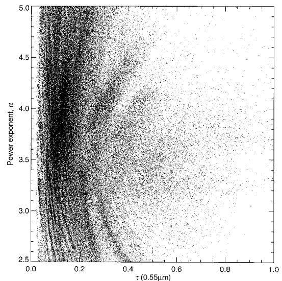
Fig. 10. Scatterplot of aerosol power exponent versus optical thickness for July 1986.
