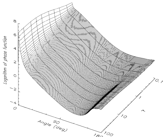
Fig. 16. Phase function versus \gamma and scattering angle for the bimodal log normal size distribution of Eq. (11) and m = 1.5 + 0.005i .
