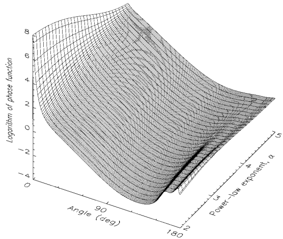
Fig. 1. Phase function versus power exponent and scattering angle for the power-law size distribution of Eq. (4) and m = 1.5 + 0.005i .
