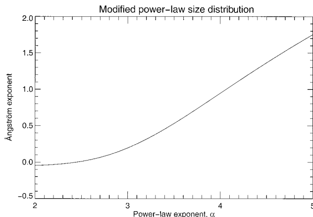
Fig. 3. Ångström exponent versus power exponent for the power-law size distribution of Eq. (4).
