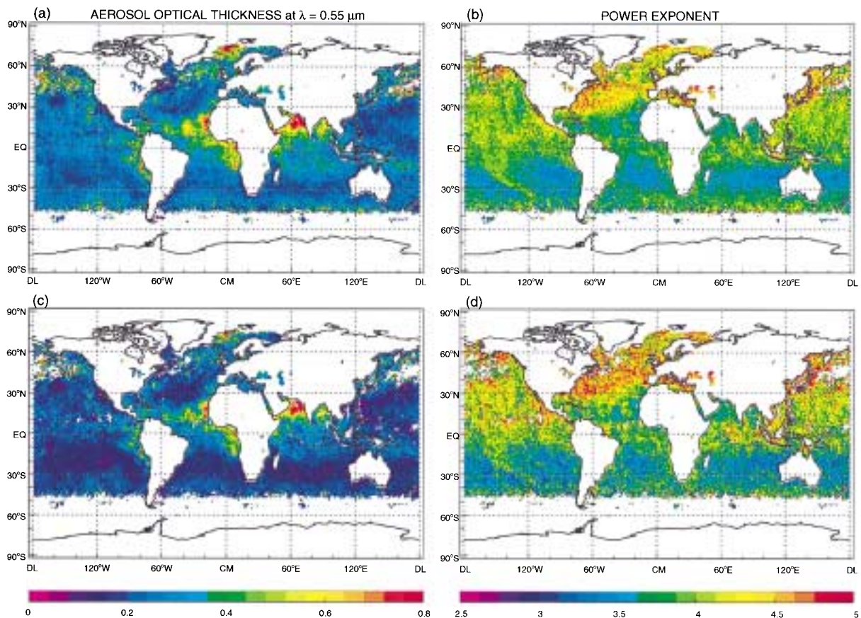
Fig. 6. (a) and (b) Monthly mean optical thickness ( \tau ) and optical-thickness-weighted power exponent ( \alpha ) for July 1986 derived with the benchmark atmosphere–ocean model and the standard ISCCP cloud-detection scheme. (c) and (d) As in panels (a) and (b) but with a modified cloud-detection scheme that retains only pixels with channel-5 temperatures warmer than the respective composite values.
