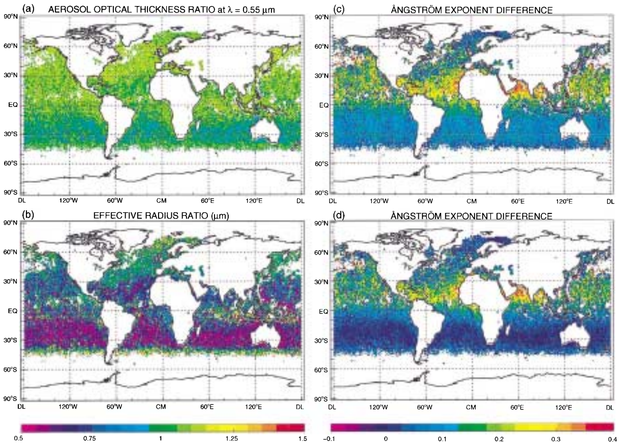
Fig. 15. (a) Ratio of monthly mean aerosol optical thicknesses retrieved with the bimodal size distribution of Eq. (11) and the modified power law of Eq. (4). (b) As in (a) but for the effective radius ratio. (c) As in (a) but for the difference of optical-thickness-weighted monthly mean Ångström exponents. (d) As in (c) but for the difference of simple monthly mean Ångström exponents.
