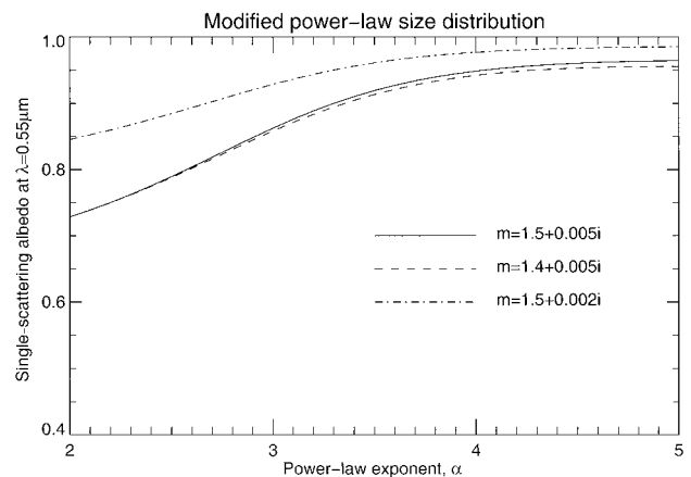
Fig. 5. Single-scattering albedo versus power exponent for the power-law size distribution of Eq. (4) and three values of the refractive index.
