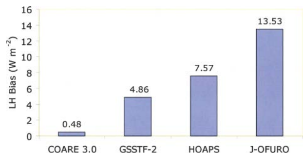
Fig. 2. Evaluation of modeled latent heat fluxes and direct flux measurements taken during the NOAA ETL and French deployments. The following bulk flux models are compared (see text): COARE 3.0, HOAPS, GSSTF-2, and J-OFURO.
