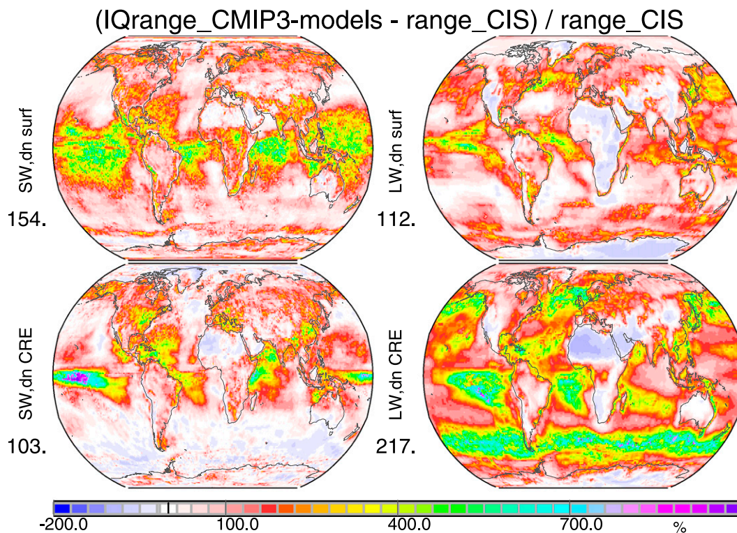
FIG. 13. Comparisons of spread ranges for downward (left) shortwave and (right) longwave radiative fluxes (top) during all-sky conditions and (bottom) contributing CRE. The local interquartile range in CMIP3 global modeling ( \Delta CMIP3) is compared with the local CIS range ( \Delta CIS) via the ratio of (\Delta CMIP3 - \Delta CIS) to ( \Delta CIS) in percent. Positive values indicate a larger diversity in the modeling. Negative values indicate a smaller diversity in the modeling. Values below the labels indicate global averages (%).
