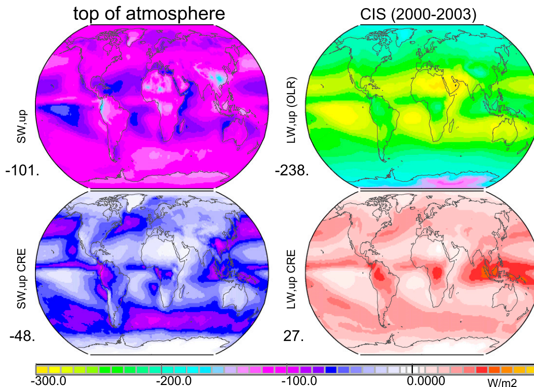
FIG. 5. Multiyear (2000–03) annual CIS radiative flux averages at the TOA for upward (left) shortwave and (right) longwave fluxes for (top) radiative fluxes at all-sky conditions and (bottom) contributing cloud impacts (CRE). Values below the labels indicate global averages. By definition all upward fluxes are negative, so that negative values of upward SW CRE refer to an increase and positive values of upward LW CRE refer to a decrease in clear-sky fluxes.
